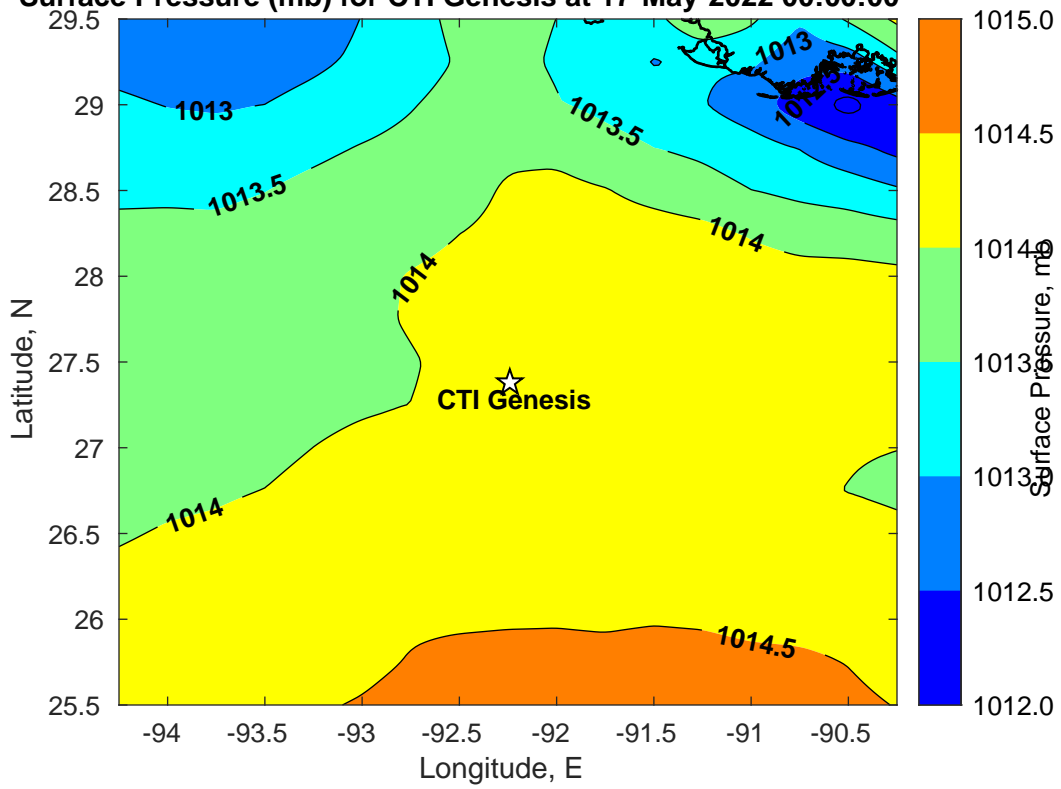
Surface Pressure (mb) for CTI Genesis at 17-May-2022 00:00:00
